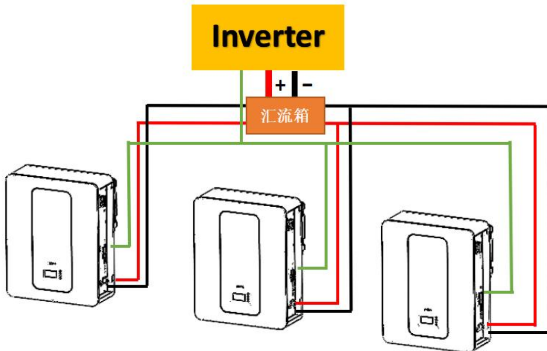
Solution 2: High power (multiple machines in parallel)
