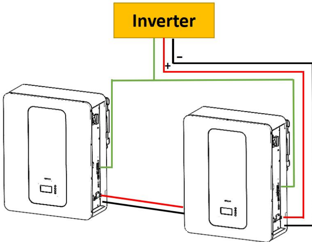
Solution 2: High power (multiple machines in parallel)
