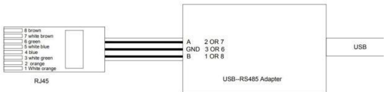
Wiring Diagram
